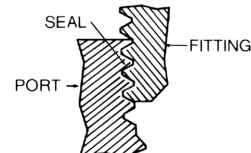
SEAL IS CREATED BY INTERFERENCE BETWEEN THREADS
