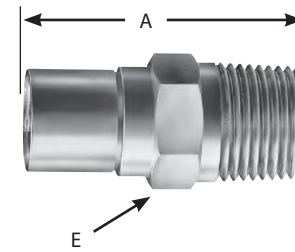
Male Pipe (NPT)
